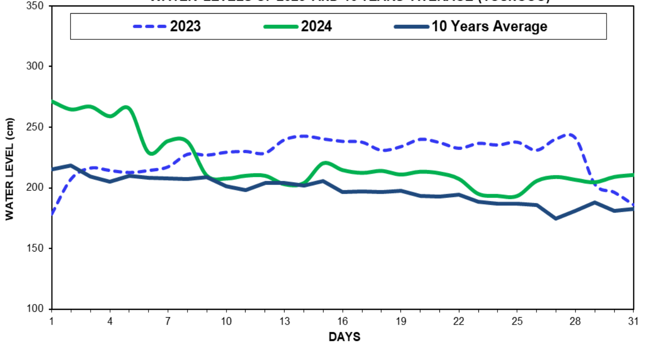
Fig(9) COMPARISON OF DECEMBER WATER LEVELS OF 2024 WITH DECEMBER WATER LEVELS OF 2023 AND 10 YEARS AVERAGE (TOUNGOO)
