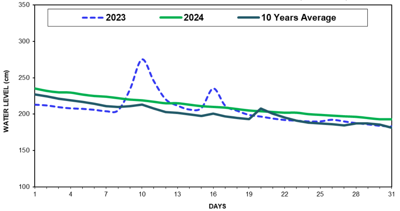
Fig(1) COMPARISON OF DECEMBER WATER LEVELS OF 2024 WITH DECEMBER WATER LEVELS OF 2023 AND 10 YEARS AVARAGE (MYITKYINA)
