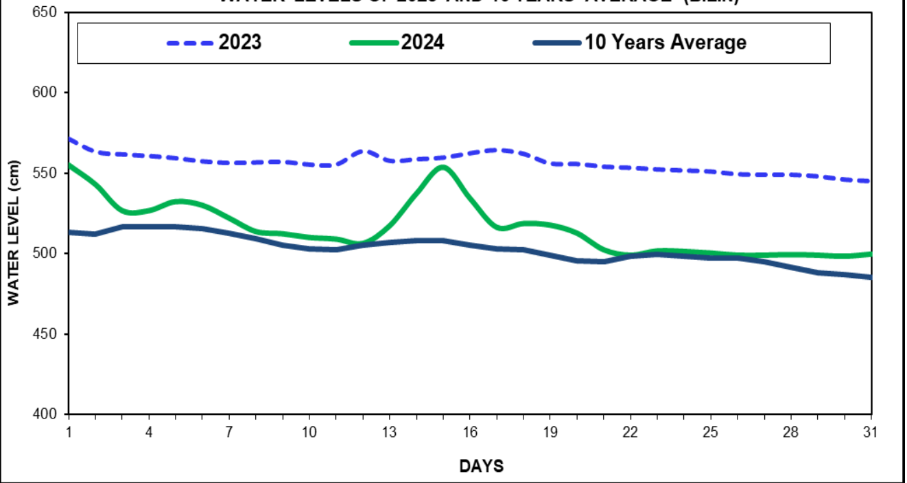
Fig(17) COMPARISON OF DECEMBER WATER LEVELS OF 2024 WITH DECEMBER WATER LEVELS OF 2023 AND 10 YEARS AVERAGE (BILIN)
