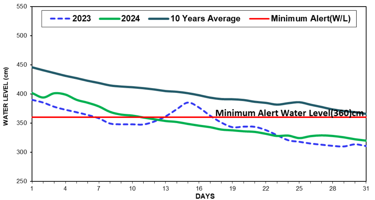
Fig(2) COMPARISON OF DECEMBER WATER LEVELS OF 2024 WITH DECEMBER WATER LEVELS OF 2023 AND 10 YEARS AVERAGE (MANDALAY)
