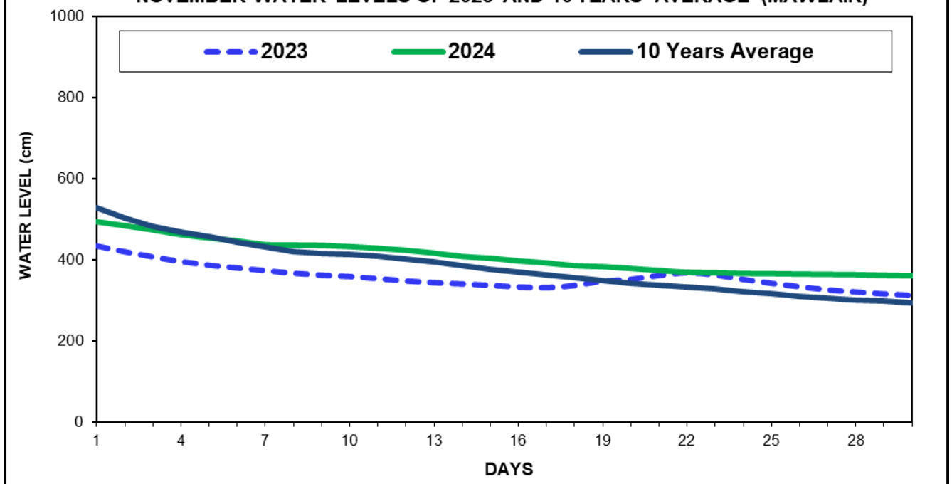
Fig(6) COMPARISON OF NOVEMBER WATER LEVELS OF 2024 WITH NOVEMBER WATER LEVELS OF 2023 AND 10 YEARS AVERAGE (MAWLAIK)
